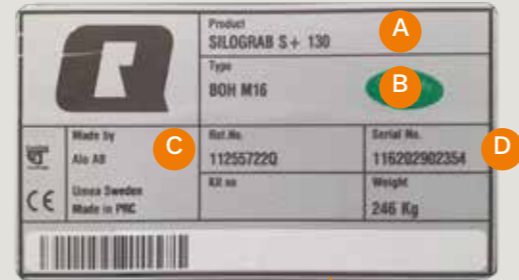
Plaque d'identification outil
